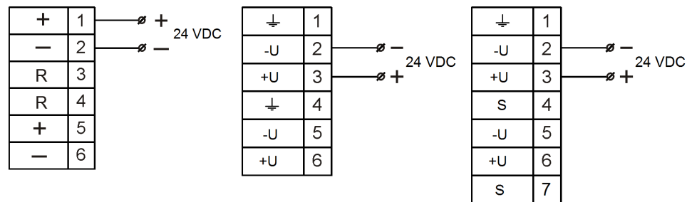
а) BC-07e-Ex-3(I)-24VDC
