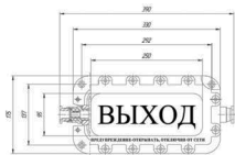
ОВ-1.01; ОВ-3.01
