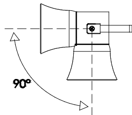
Fig. 2 Speaker orientation
