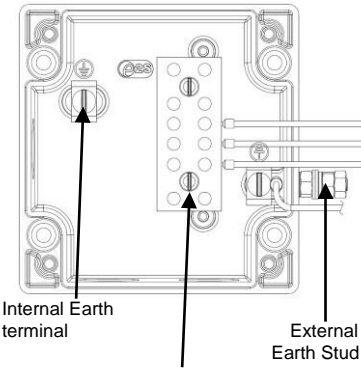
Ex e terminal block
